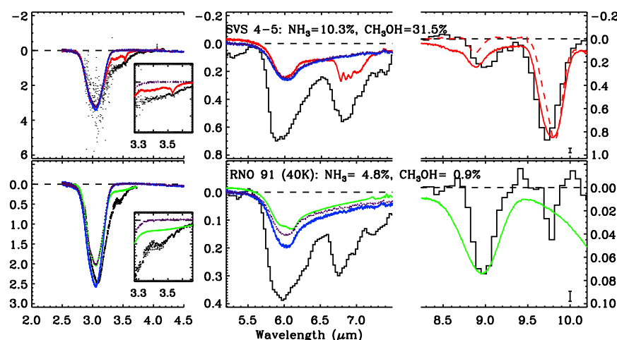
Figure 3.13 Comparison of astronomical data (VLT or Keck measurements at short wavelengths, IRS Spitzer observations elsewhere) and laboratory spectra in selected wavelength ranges: 2.0–4.5 \mu m (left panels), 5.2–7.5 \mu m (middle panels) and 8.2–10.2 \mu m (right panels, silicate absorption subtracted via the template method). Error bars are indicated in the bottom-right corner. Overlaid in red and green are laboratory spectra corresponding to H 2 O:CH 3 OH:NH 3 =10:4:1 and H 2 O:NH 3 =9:1, respectively, scaled to the 9 \mu m NH 3 umbrella mode. The dark blue line represents the pure water laboratory spectrum scaled to the water column density taken in paper I. The dotted purple line corresponds to a pure water spectrum scaled to the 3 \mu m water feature of the mixed ice spectrum, showing the contribution of NH 3 features around 3.47 and 6.1 \mu m. Finally, the red dashed line in the right panel of SVS 4-5 represents a H 2 O:CH 3 OH=9:1 laboratory spectrum scaled to the 9.7 \mu m CH 3 OH CO-stretch mode: this gives an indication of the contribution of the 9 \mu m CH 3 OH CH 3 -rock mode to the total 9 \mu m feature. The laboratory spectra are recorded at 15 K unless indicated differently.
