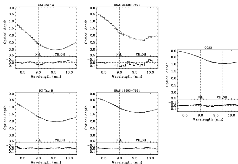
Figure 3.4 Silicate features of the sources used as templates for a straight 8 \mu\text{m} wing (left), curved 8\text{-}\mu\text{m} wing (middle), and GCS3 (right). The bottom panels of each plot are the residuals after removal of the local continuum shown in grey in the top panels. The optical depth scale is kept fixed for comparison. These sources are selected to have no or at most weak \text{NH}_3 and \text{CH}_3\text{OH} absorptions.
