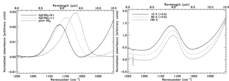
Figure 3.6 ( Left ) FTIR ice spectra of the \nu_{\text{NH}_3} mode for pure NH 3 , a H 2 O:NH 3 =1:1 and a H 2 O:NH 3 =9:1 mixture at a temperature of 15 K. At the low frequency side of the spectrum the H 2 O libration mode (centered around 770 cm -1 , or 13 μm) starts showing up for the H 2 O-containing mixtures. — ( Right ) Temperature effect on a H 2 O:NH 3 =9:1 mixture: decreasing FWHM with increasing temperature.
