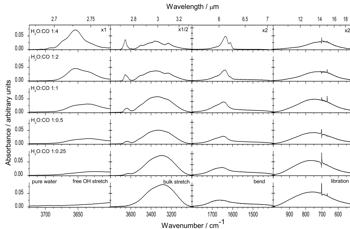
Figure 2.2 Combined spectra of the four modes for water ice for the six measured compositions (see Table 2.1), ranging from pure water ice (bottom) to a 1:4 H 2 O:CO mixture (top figures). The spectra are taken at a temperature of 15 K. Note that the wavelength ranges for separate modes are different. The small structures on the libration mode are experimental artifacts.
