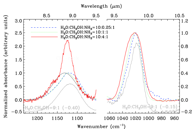
Figure 3.10 Normalized spectra of the \text{CH}_3\text{OH} \nu_4 \text{C}-\text{O} mode (right panel), and \text{NH}_3 \nu_2 umbrella mode (left panel) for a \text{H}_2\text{O}:\text{CH}_3\text{OH}:\text{NH}_3=10:0.25:1 , a \text{H}_2\text{O}:\text{CH}_3\text{OH}:\text{NH}_3=10:1:1 and a \text{H}_2\text{O}:\text{CH}_3\text{OH}:\text{NH}_3=10:4:1 mixture at a temperature of 15 K. These mixture ratios span the range of observed interstellar column density ratios. Spectra were normalized to better show the changes in band maximum position and FWHM of each feature. Spectra of a \text{H}_2\text{O}:\text{CH}_3\text{OH}=9:1 and a \text{H}_2\text{O}:\text{NH}_3=1:1 mixture were offset and overlaid in light grey in the right and left panel, respectively. In the case of \text{H}_2\text{O}:\text{CH}_3\text{OH}:\text{NH}_3=10:4:1 , the \text{NH}_3 \nu_2 umbrella mode is heavily blended with the \text{CH}_3\text{OH} \nu_7 \text{CH}_3 rocking mode, so that the dark grey line actually shows the Gaussian fit to the underlying \text{NH}_3 feature, whereas the full 9\text{ }\mu\text{m} feature is shown in black.
