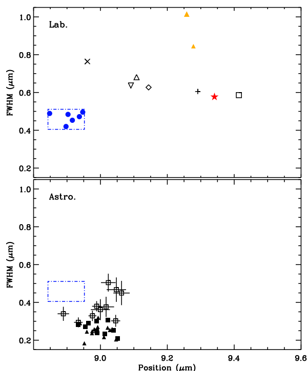
Figure 3.11 FWHM and band maximum position of the NH 3 feature measured in the laboratory mixtures at 15 K (“Lab.”, top panel) and in the Spitzer spectra (“Astro.”, bottom panel). In the top panel, the filled star indicates pure NH 3 , filled circles represent H 2 O-rich mixtures and filled triangles are for NH 3 :CH 3 OH mixtures (an increasing symbol size indicative of increasing CH 3 OH content). Other symbols are as follows: + for NH 3 :H 2 O=1:0.11, ∇ for NH 3 :H 2 O=1:1, ◇ for NH 3 :H 2 O:CO=1:1:1, △ for NH 3 :H 2 O:CO 2 =1:1:1, □ for NH 3 :CO:CO 2 =1:1:1, × for NH 3 :CH 3 OH:H 2 O=1:1:1. In the bottom panel, open and filled squares indicate values obtained with the template and local continuum method, respectively. The dash-dot polygons delimitate the parameter space of FWHM and positions corresponding to H 2 O-rich mixtures.
