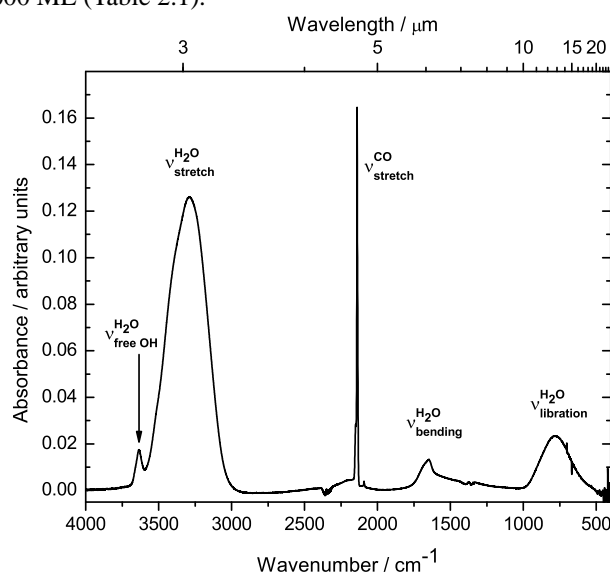
Figure 2.1 A typical baseline and background corrected ice spectrum for a H 2 O:CO=1:1 mixture. The measurement is performed at 15 K. The vibrational modes in the H 2 O:CO ice are indicated.
