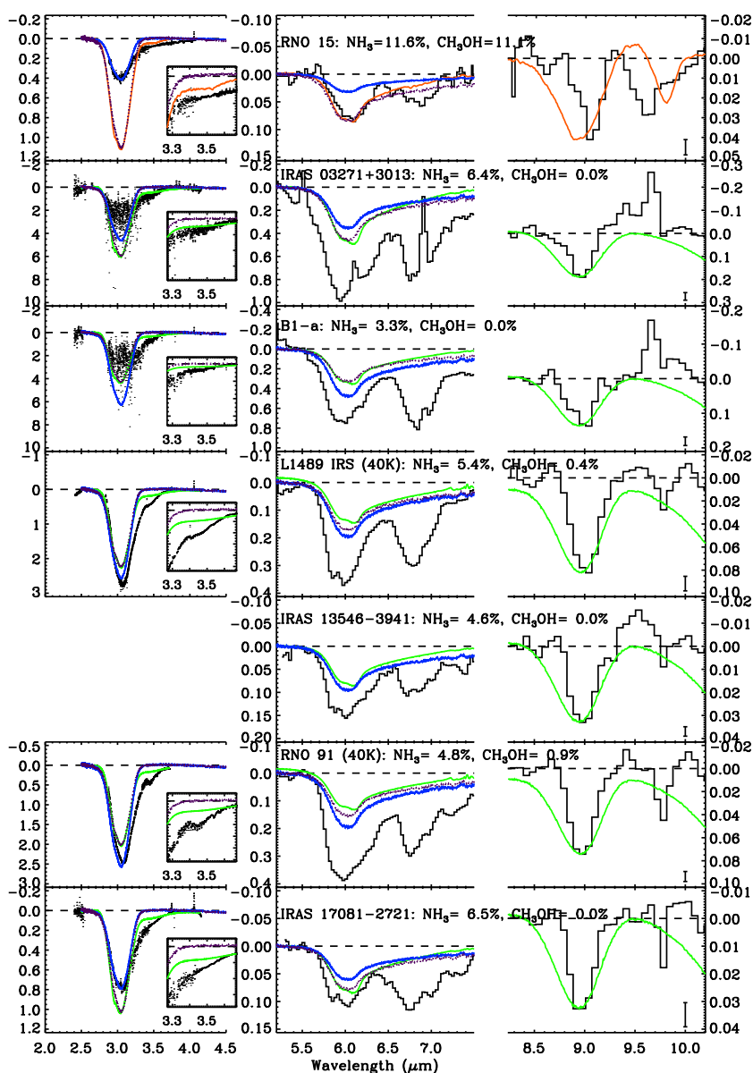
Figure 3.15 (b) As for Fig. 3.14 but for sources with no associated template, i.e. with the 10 μm silicate feature subtracted via the local continuum method. Additionally, yellow represents H 2 O:NH 3 =4:1 (H. Fraser, priv. comm.).
