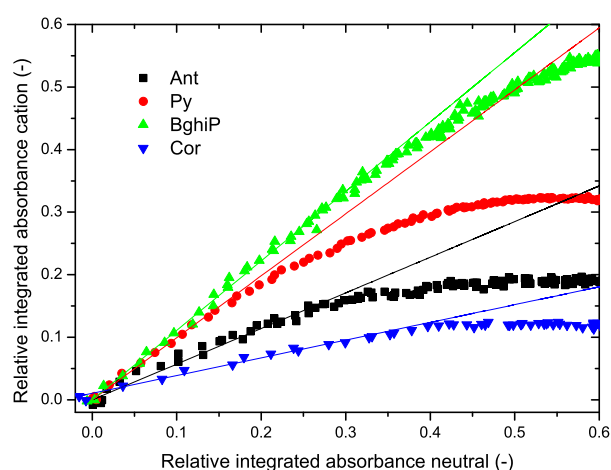
Figure 7.1 The correlation between the amount of produced cation and the amount of used neutral, both relative to the total deposited amount of neutral PAH.
