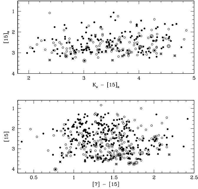
Figure 2.9: Lower panel: [15] versus ([7] - [15]) colour-magnitude diagram; where ISOGAL magnitudes, or the A and D MSX magnitudes if no ISOGAL magnitude is available, are used. Upper panel: [15]_o versus (K_o - [15]_o) ISOGAL-DENIS extinction corrected colour-magnitude diagram. Detections are shown as filled circles; non-detections as open circles. The LPVs from Glass et al. (2001) are marked with a larger open circle, whereas the sources from Schultheis et al. (2000) are marked with crosses. Note that two points fall outside the figure.
