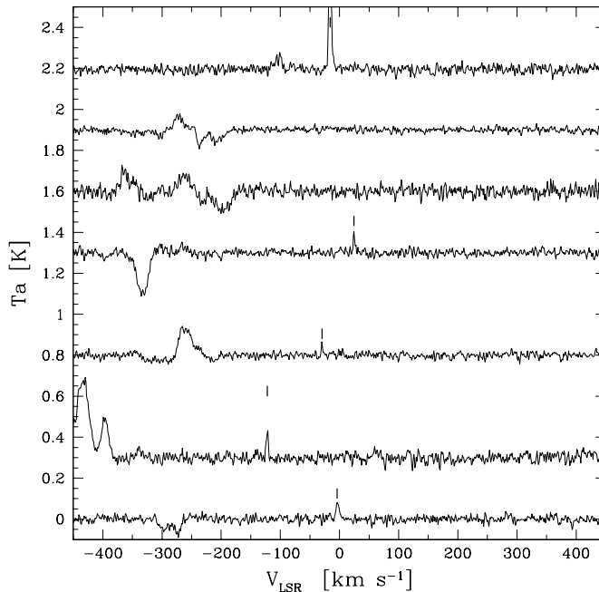
Figure 2.5: Some spectra with interstellar H^{13}CN emission, shown for clarity with arbitrary antenna temperature offsets. The small thick vertical bars indicate the detected SiO maser line. The H^{13}CN and SiO lines are usually clearly distinct.
