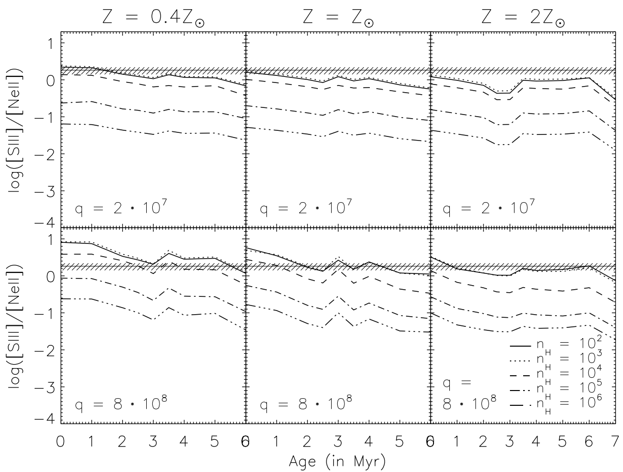
Fig. 8. Same as Fig. 7, but now for the emission line ratio [\text{S III}]_{18.71\mu\text{m}}/[\text{Ne II}]_{12.81\mu\text{m}} .
