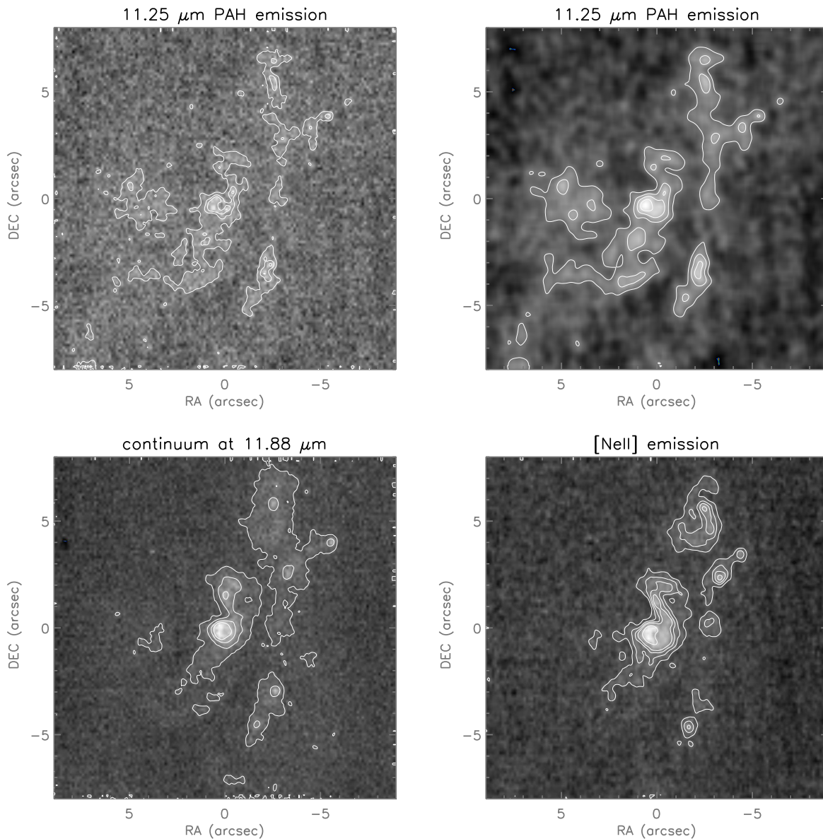
Fig. 1. Mid-infrared images of the nucleus of M83, all based on narrow-band observations obtained with VISIR. The upper two panels show the continuum-subtracted PAH emission at 11.25 \mu\text{m} . Upper left: the PAH emission is shown after rebinning the image onto a finer grid, interpolating the pixel values in steps of 1/10 of the pixel size. The contours correspond to 1.0 , 1.7 , and 2.2 \cdot 10^{-13} \text{ erg s}^{-1} \text{ cm}^{-2} \text{ arcsec}^{-2} (in all images the lowest contours corresponds to 5\sigma above the background). Upper right: is the same image as the upper left, but the technique of adaptive filtering is applied with a kernel of 5 pixels to remove the high frequency noise (Lorenz et al, 1993). The contours in this image correspond to 0.8 , 1.3 , 1.7 , and 2.2 \cdot 10^{-13} \text{ erg s}^{-1} \text{ cm}^{-2} \text{ arcsec}^{-2} . The bottom row shows left: the continuum at 11.88 \mu\text{m} (the PAH2.2 filter, the other continuum images show similar morphology), and right: the continuum-subtracted [Ne II] image. Both images are rebinned in the same way as the upper left PAH map. The contours correspond to 21.7 , 55.8 , 93.0 , and 124.0 \text{ mJy arcsec}^{-2} in the continuum map and to 2.2 , 3.2 , 4.8 , 6.0 , and 9.0 \cdot 10^{-13} \text{ erg s}^{-1} \text{ cm}^{-2} \text{ arcsec}^{-2} in the [Ne II] image. In all images North is up and East is left. The x- and y-axes are in arcsec and (0,0) corresponds to (\alpha, \delta) = (13 \text{ }^{\text{h}} 37 \text{ }^{\text{m}} 00.538 \text{ s}, -29 \text{ }^{\circ} 51 \text{ }^{\prime} 54.81 \text{ }^{\prime\prime}) . The optical nucleus is located at (\Delta\alpha, \Delta\delta) = (+5^{\prime}.7, +0^{\prime}.85) , left of the brightest mid-infrared peak in the images shown here.
