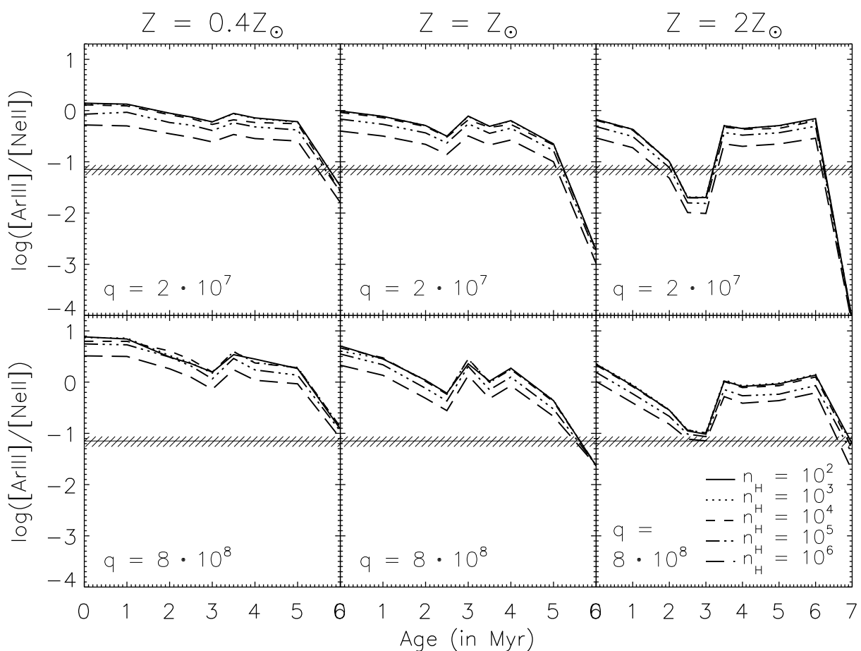
Fig. 7. Evolution of the emission line ratio [\text{Ar III}]_{8.99\mu\text{m}}/[\text{Ne II}]_{12.81\mu\text{m}} with cluster age. The left panels show the curves for Z = 0.4Z_{\odot} , the middle panels Z = Z_{\odot} and the right panels Z = 2Z_{\odot} . The upper row shows the case of low ionization parameter, q = 2 \cdot 10^7 \text{ cm s}^{-1} , the lower row that of high ionization parameter, q = 8 \cdot 10^8 \text{ cm s}^{-1} . Curves of different line style represent results of models with different densities, ranging from 10^2 \text{ cm}^{-3} to 10^6 \text{ cm}^{-3} . Line ratio values can be found tabulated at www.ifa.hawaii.edu/kewley/Mappings/IRdiagnostics . The ratio value measured from the spectrum of the central mid-infrared source in the nucleus of M83 is overplotted in all panels (horizontal solid line), the magnitude of the error is indicated by the dashed region.
