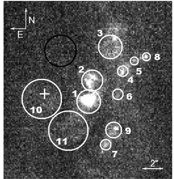
Fig. 3. The positions and sizes of the apertures for photometry on an image in the PAH2 filter (continuum plus PAH emission). Apertures 1 – 9 correspond to the compact knots identified in the [Ne II] and continuum images. Positions 10 and 11 correspond to regions of diffuse emission. The black aperture indicates where the local background was measured. The white cross indicates the location of the optical nucleus.
