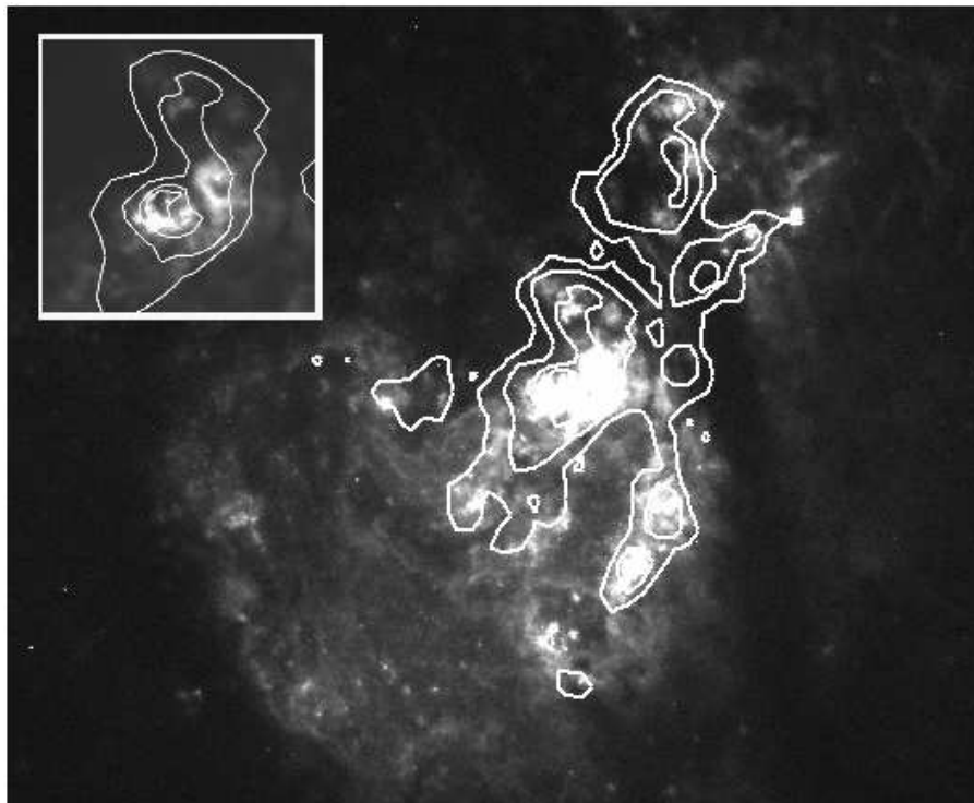
Fig. 4. Emission in the [Ne II] filter ([Ne II] lines emission plus continuum) overlaid in white contours on a HST F656N image ( H\alpha emission plus continuum). The contours correspond to 1.7, 3.2, 6.9, 13.6 and 19.1 \cdot 10^{-13} \text{ erg s}^{-1} \text{ cm}^{-2} \text{ arcsec}^{-2} . Astrometric calibration of the mid-infrared images is done by matching the position of the brightest peak with that of the brightest peak in the Spitzer 8 \mu\text{m} IRAC image. Inserted: a blow-up of the region around the brightest mid-infrared peak (source 1). Note how the [Ne II] emission follows the ring-like distribution observed in the F656N image.
