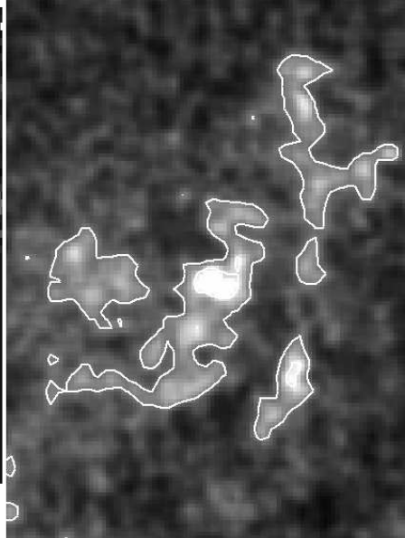
Fig. 5. A comparison of left : near-infrared H 2 1-0 S(1) emission (2.1218 \mu\text{m} ) measured with the integral field spectrograph SINFONI, middle : 11.25 \mu\text{m} PAH emission, and right : 12.81 \mu\text{m} [Ne II] fine-structure line emission. The contours correspond to PAH emission at 0.9 and 1.7 \cdot 10^{-13} \text{erg s}^{-1} \text{cm}^{-2} \text{arcsec}^{-2} . Note how the PAH emission traces the distribution in the [Ne II] emission much closer, than the H 2 emission does.
