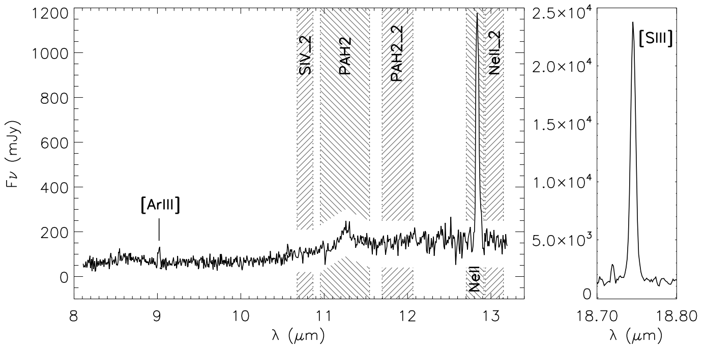
Fig. 2. Left: Low-resolution N-band spectrum of the brightest mid-infrared source in the nucleus of M83 (source 1). The dashed vertical bands indicate the wavelength range covered by the narrow-band imaging filters. The names of the imaging filters are indicated as well. Right: Medium-resolution Q-band spectroscopy covering the range between 18.7 – 18.8 \mu\text{m} of the same source. The feature at 18.714 \mu\text{m} results from an array artefact.
