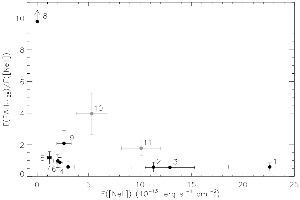
Fig. 6. In this diagram the strength of the PAH flux F(\text{PAH}_{11,25}) relative to the [\text{Ne II}] flux F([\text{Ne II}]) is plotted versus F([\text{Ne II}]) . The black symbols correspond to the compact knots, sources 1 – 9, and the grey to the regions of diffuse emission, sources 10 and 11. The compact knots defined in the [\text{Ne II}] map, sources 1 – 7, all have a very similar F(\text{PAH}_{11,25})/F([\text{Ne II}]) ratio. The compact sources defined from continuum peaks and the diffuse sources have much stronger PAH emission relative to the [\text{Ne II}] emission. Source 8 clearly stands out with a very large F(\text{PAH}_{11,25})/F([\text{Ne II}]) ratio.
