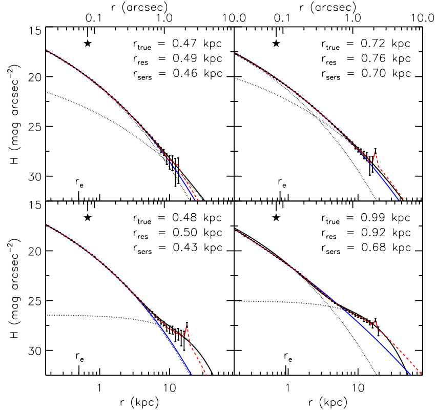
Figure 3. Residual-corrected fits to simulated galaxy images (red curves). Top: compact n = 4 profile and extended n = 4 profile, with flux ratios 10 : 1 (left) and 2 : 1 (right). Bottom: compact n = 4 profile and extended n = 1 profile, with the same flux ratios as in the top panels. At large radii, where uncertainties in the sky determination become significant, the profile is extrapolated. This is indicated by dashed curves. The solid black curves indicate the total intrinsic surface brightness profiles, the dotted black curves indicate the individual components that make up these profiles. The best-fit uncorrected Sérsic profiles are shown as blue curves. These deviate strongly from the true profiles at large radii. The residual-corrected profiles (red curves) follow the intrinsic profiles extremely well, demonstrating that our method recovers the intrinsic profiles accurately; the derived effective radii, indicated on the bottom x -axes, are within 10% of the true effective radii. The PSF size (HWHM) is indicated by the star symbols on the top x -axes.
