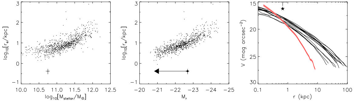
Figure 4. Relations between size and stellar mass (left) and size and rest-frame r -band luminosity (middle) for a sample of low-redshift galaxies, taken from Guo et al. (2009). The large symbol with error bars indicates the position of the galaxy of our study. Low-redshift galaxies are much larger at similar stellar masses and luminosities. The arrow in the middle plot indicates the change in luminosity due to passive evolution to z = 0 . The size of the galaxy is smaller than the local equivalents by a factor of 10. Right: comparison of best-fit residual-corrected rest-frame V -band surface brightness profile (red curve) to elliptical galaxies in the Virgo cluster, from Kormendy et al. (2009; black curves). Virgo galaxies are plotted with M_*/M_\odot > 10^{11} . The observed high- z surface brightness profile has been corrected for cosmological surface dimming and passive M/L evolution from z = 1.91 to z = 0 (see the text). Assuming the galaxy has a mass > 10^{11} M_\odot at z = 0 , its profile at large radii will evolve very strongly over the next 10 Gyr. The central surface brightness profile, on the other hand, shows much less evolution between z \approx 2 and z = 0 .
