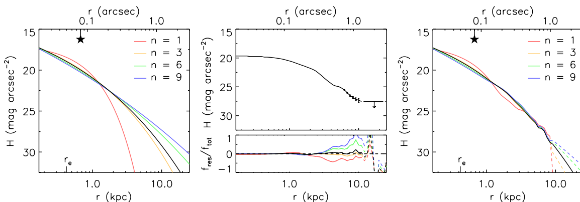
Figure 2. Our method of correcting the observed surface brightness profile for the effects of the HST WFC3 PSF and incorrect profile modeling. In the left panel the best-fitting Sérsic models, derived from a two-dimensional fit using a star as the PSF, are shown for different values of n . The black curve indicates the free- n fit, with n = 3.7 . The profiles show large variations. In the top center panel the observed profile is shown. The residual fluxes from the Sérsic fits are shown in the bottom panel as a fraction of the observed flux. In the right panel the profiles derived using our “residual-correction” method are shown. At large radii, where uncertainties in the sky determination become significant, the profile is extrapolated. This is indicated by dashed curves. The residual-corrected profiles are much more robust to modeling errors than the uncorrected profiles. The derived effective radius is indicated on the bottom x -axis, the PSF size (HWHM) is indicated by the star symbol on the top x -axis. The solid horizontal line in the middle panel indicates the 3\sigma sky noise level. As can be seen, the surface brightness profile can be robustly measured to a surface brightness of 28 \text{ mag arcsec}^{-2} .
