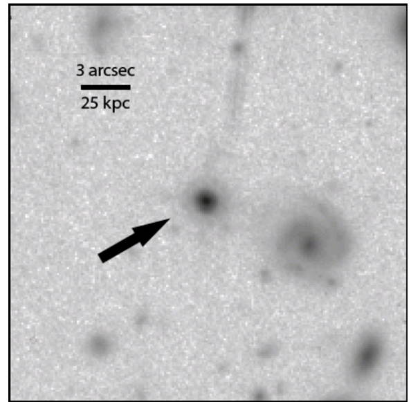
Figure 1. WFC3 H_{F160W} -band image of the galaxy. It is well separated from its nearest neighbors.
