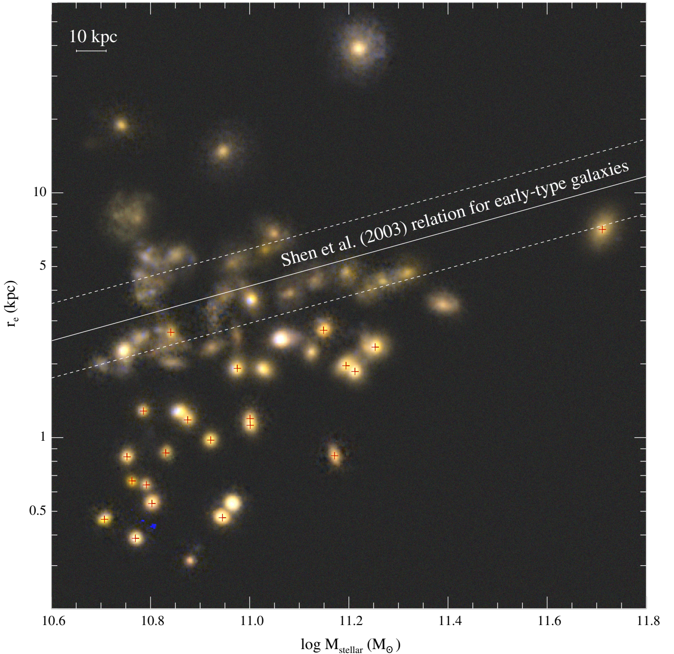
Figure 2. Stellar masses and sizes of galaxies at 1.5 < z < 2.5 with M_{\text{stellar}} > 5 \times 10^{10} M_{\odot} . Color images are composed of rest-frame U_{336} , B_{438} , and g_{475} images, obtained from observed I_{814} , J_{125} , and H_{160} images. Galaxies which are included in our quiescent sample are indicated with red crosses. Although we do not select based on morphology, almost all galaxies in our quiescent sample are compact, bulge-dominated, and have red colors.
