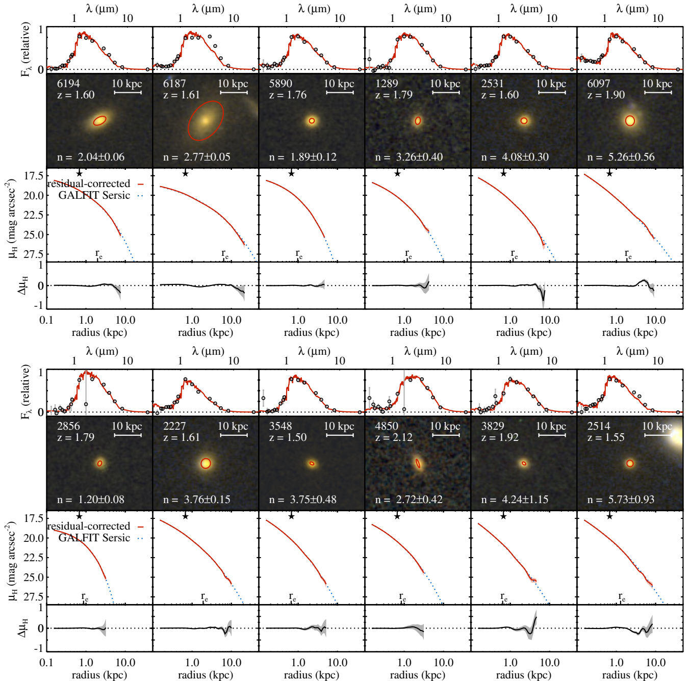
Figure 4. Broadband SEDs, color images, and PSF-corrected surface brightness profiles of z \sim 2 quiescent galaxies. The SEDs, obtained with FAST (Kriek et al. 2009), are based on photometry from the FIREWORKS catalog. The color images are composed of rest-frame U_{336} , B_{438} , and g_{475} images, obtained from the observed I_{814} , J_{125} , and H_{160} data. The red ellipses are constructed from the best-fitting effective radii, axis ratios, and position angles. The best-fit Sérsic profiles, obtained using GALFIT, are indicated by blue dotted curves. Residual-corrected surface brightness profiles are shown in red. Effective radii and the PSF HWHM are indicated at the bottom and top axes, respectively. We are able to measure the true surface brightness profiles of these galaxies down to approximately 26 \text{ mag arcsec}^{-2} and out to r \approx 10 \text{ kpc} . In the bottom row, we show the difference between the best-fit Sérsic profile and the residual-corrected profile. Individual residual-corrected profiles show deviations from simple Sérsic profiles, although these deviations are consistent with zero within the errors.
