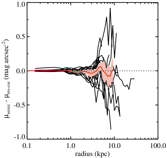
Figure 5. Deviations of galaxy profiles from Sérsic profiles. The difference between the best-fit Sérsic profile and the residual-corrected profile is plotted as a function of radius for all galaxies in our sample (black lines). The mean profile is shown in red, with the shaded light red region indicating the 1\sigma spread in the distribution. Although individual galaxy profiles deviate from Sérsic profiles, on average the difference is consistent with zero.
