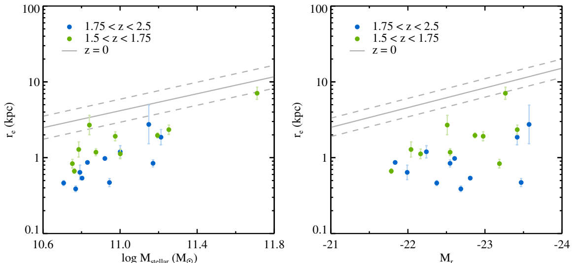
Figure 6. Relations between size and stellar mass (left panel) and size and rest-frame r -band absolute magnitude (right panel). Gray lines indicate the low-redshift mass–size and magnitude–size relations from Shen et al. (2003), green and blue points indicate the z \sim 2 sample (divided into low- and high-redshift bins, respectively). The z \sim 2 galaxies are, on average, almost an order of magnitude smaller than low-redshift galaxies of similar mass and luminosity. However, there is a significant range in sizes at both redshifts. The largest z \sim 2 galaxies lie very close to the z = 0 mass–size relation.
