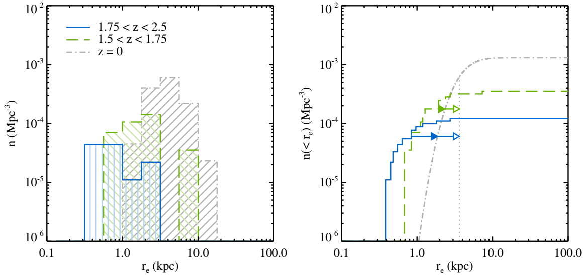
Figure 9. Comoving number density (left panel) and cumulative comoving number density (right panel) as a function of effective radius r_e , for galaxies at 1.75 < z < 2.5 , 1.5 < z < 1.75 , and z = 0 (solid blue, dashed green, and dot-dashed gray lines, respectively). The z = 0 number densities are obtained by combining the stellar mass function of Bell et al. (2003) with the mass–size relation of Shen et al. (2003). The z \sim 2 number densities have been scaled such that the total number density corresponds to the results of Brammer et al. (2011). Both the median effective radius and the total number density of quiescent galaxies show a strong increase from z \sim 2 to z = 0 . The solid arrows in the right-hand panel indicate the minimum size growth required for high-redshift galaxies to grow into the smallest galaxies at z = 0 . The open arrows indicate the size growth required for high-redshift galaxies to grow to the same median size as galaxies at z = 0 . The minimum size growth required for z \sim 2 quiescent galaxies is approximately a factor two smaller than the median size growth between z \sim 2 and z = 0 .
