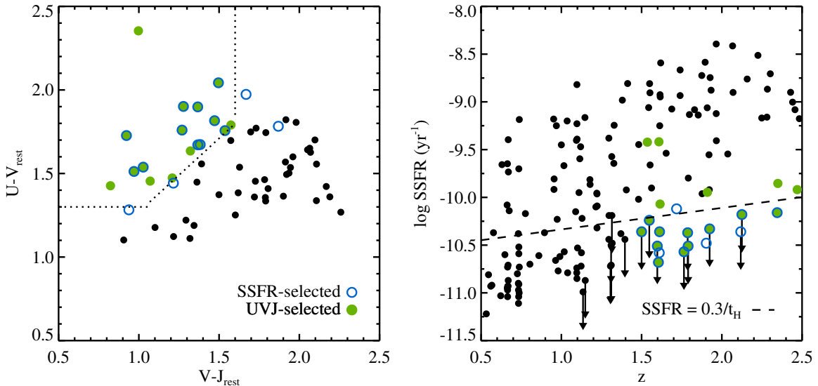
Figure 1. Left panel: rest-frame U-V and V-J colors of galaxies in the CANDELS GOODS-South deep field at 1.5 < z < 2.5 . Right panel: specific star formation rates as a function of redshift. Arrows indicate upper limits. The dashed line indicates where the specific star formation rate is equal to 0.3/t_H . Quiescent galaxies selected using the UVJ color criterion are shown as filled green circles. Galaxies which are selected as quiescent based on their SSFRs are shown as open blue circles. There is good agreement between the two selection criteria. Both the UVJ -selected galaxies and the SSFR-selected galaxies are included in our quiescent galaxy sample.
