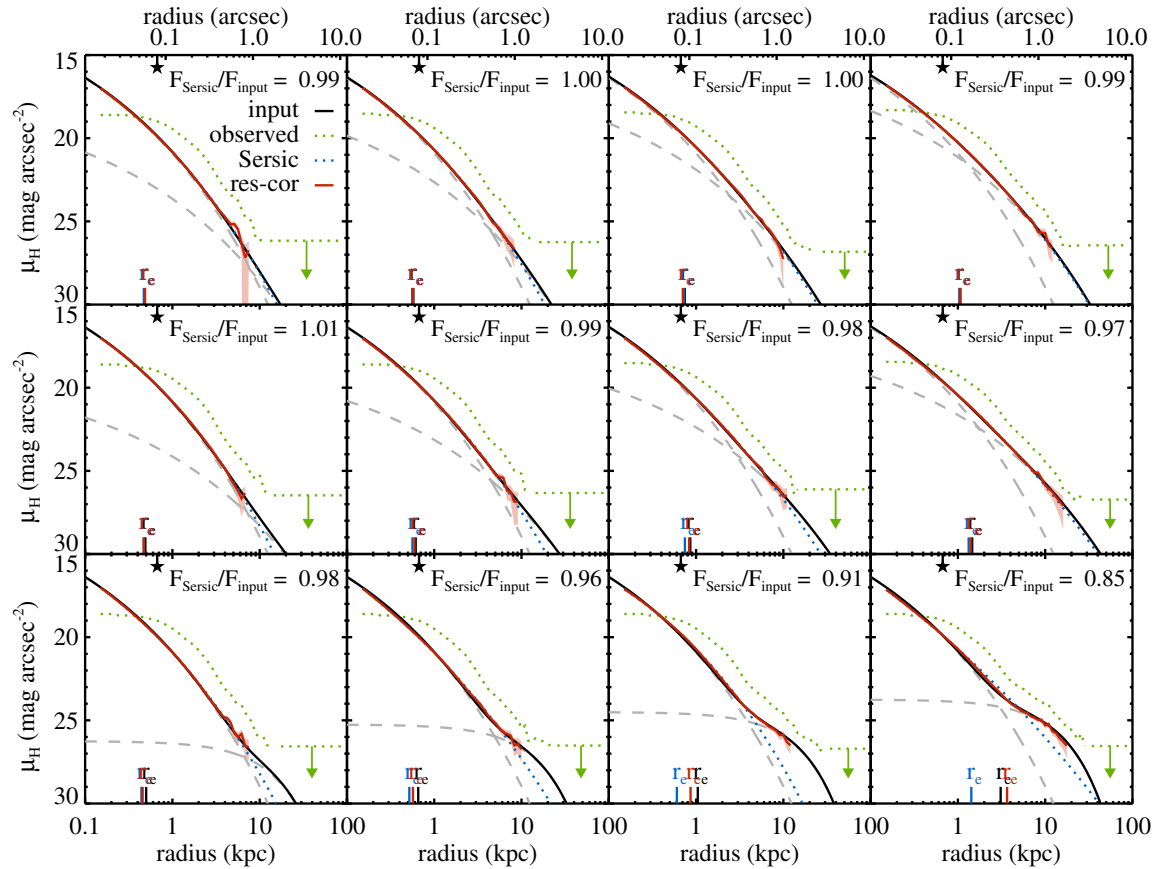
Figure 3. Effectiveness of the residual correction for recovering surface brightness profiles. The method was tested on a large number of simulated galaxies, composed of two components: one compact bright component and an extended fainter component. A small selection is shown here. The input profiles are shown in black, with the dashed gray lines indicating the two subcomponents. The PSF-convolved “observed” profiles are shown in green. Direct Sérsic fits are shown in blue, and the residual-corrected profiles are overplotted in red. The shaded light red regions indicate the 1\sigma errors due to uncertainty in the sky estimation. The size of the PSF half-width at half-maximum (HWHM) is indicated on the top axis of each panel. Input effective radii are indicated in black on the bottom axes. Effective radii derived from the direct Sérsic fits and from the residual-corrected profiles are indicated in blue and red, respectively. The fraction of the input flux within 10 kpc recovered by the Sérsic fits F_{\text{Sersic}}/F_{\text{input}} is given in each panel. The residual-corrected profiles clearly reproduce the input profiles more accurately than the simple Sérsic fits, especially at large radii.
