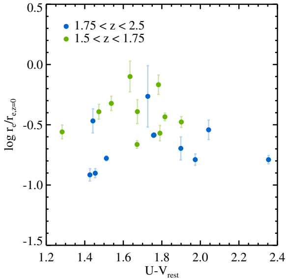
Figure 7. Offset from the z = 0 mass–size relation as a function of rest-frame U - V color for galaxies at 1.5 < z < 1.75 (green points) and 1.75 < z < 2.5 (blue points). The offset is calculated by dividing the effective radius of each galaxy by the median effective radius of z = 0 quiescent galaxies with the same mass, using the z = 0 mass–size relation from Shen et al. (2003). The galaxies are split into two redshift bins. Assuming that rest-frame U - V color is a good proxy for the mean stellar age of galaxies, we find no evidence for a correlation between galaxy compactness and galaxy age for z \sim 2 quiescent galaxies.
