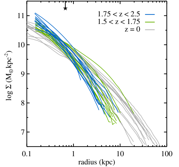
Figure 8. Comparison of stellar mass surface density profiles of z \sim 2 galaxies (blue and green curves) to elliptical galaxies in the Virgo Cluster (Kormendy et al. 2009; gray curves). The Virgo galaxies are selected to have masses equal to or higher than those of the high-redshift galaxies. Radial color gradients are ignored when calculating the mass density profiles. The star, top left, indicates the PSF HWHM at z = 2 . The central densities of the z \sim 2 galaxies are very similar to those of the z = 0 galaxies. At larger radii, however, significant evolution must occur if the z \sim 2 galaxies are to evolve into massive low-redshift elliptical galaxies.
