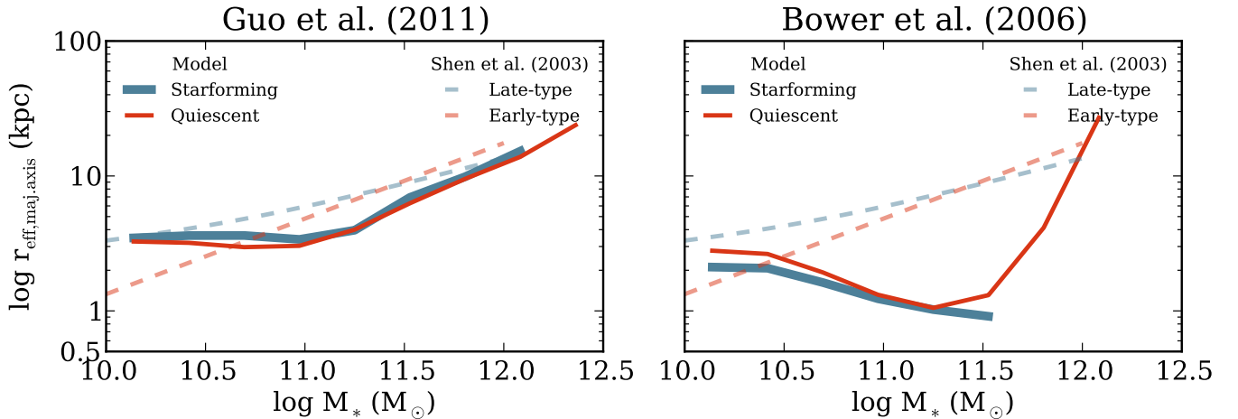
Figure 3. Median z = 0 mass-size relations for urz -selected quiescent (red) and starforming (blue) galaxies in the Guo et al. (2011) and Bower et al. (2006) models. Observations from Shen et al. (2003) are shown as dashed lines (observed values have been corrected from circularized to major-axis radii). Starforming and quiescent galaxies lie on very similar mass-size relations in both models, which is in agreement with observations in this mass range. The observed slope of the mass-size relation is reasonably well reproduced by the Guo et al. (2011) model, but the Bower et al. (2006) model incorrectly produces a negative slope.
