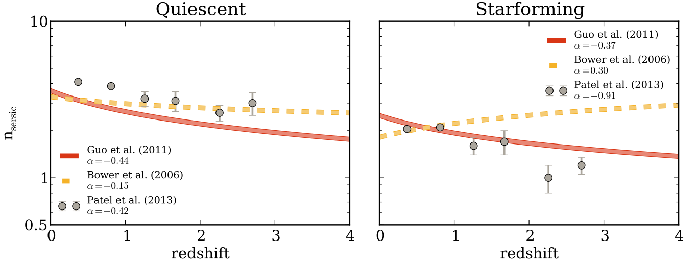
Figure 5. Evolution in the mean Sérsic index of galaxies with stellar masses 10^{10.5} < M_*/M_\odot < 10^{12} . Red (solid) and yellow (dashed) lines indicate predictions from the Guo et al. (2011) and Bower et al. (2006) models, and observed values from Patel et al. (2013) are indicated by the grey data points. Error bars indicate the errors on the median values. Best-fit \alpha parameters from (1+z)^\alpha power law fits are shown. The Guo et al. (2011) model performs very well, predicting Sérsic indices that are very close to observations both in terms of their absolute value and their relative increase with time. The Bower et al. (2006) model correctly predicts the increase in Sérsic index for quiescent galaxies, but does not match the observations for starforming galaxies.
