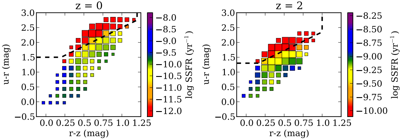
Figure 1. u-r versus r-z colors for massive ( 10^{10.5} < M_*/M_\odot < 10^{11} ) galaxies from the Guo et al. 2011 SAM catalog, at z=0 and z=2 . Color coding indicates SSFR. The dashed lines indicate our quiescent galaxy selection limits. Quiescent galaxies in the models occupy a well-defined region in the urz plane, and can be effectively selected using a two-color selection.
