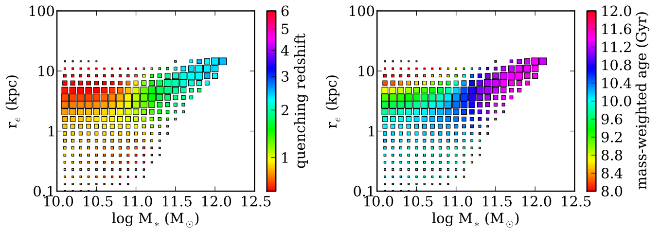
Figure 9. Mean quenching redshifts and mass-weighted ages for quiescent galaxies at z = 0 , as a function of stellar mass and size. High-mass galaxies are on average older and have quenched earlier than low-mass galaxies. At low masses there is a trend between age with size, such that smaller galaxies are on average older than larger galaxies.
