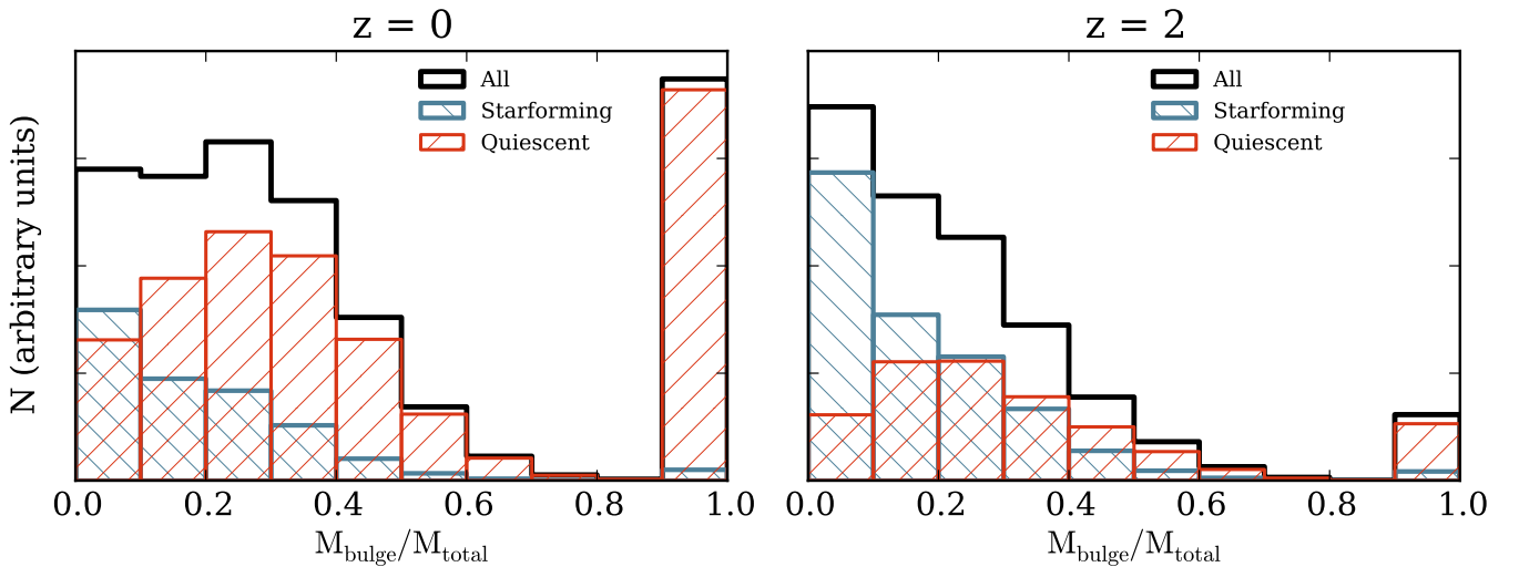
Figure 2. The distribution of bulge-to-total mass ratios for quiescent galaxies, starforming galaxies, and all galaxies (red, blue and black histograms, respectively) in the Guo et al. (2011) catalog, with stellar masses 10^{10.5} < M_*/M_\odot < 10^{11} . The distributions are shown at z=0 and z=2 . The distribution of bulge-to-total ratios is very broad, both for quiescent and starforming galaxies. This is the case at all redshifts up to z=6 . The median bulge fraction of quiescent galaxies is quite, even at low redshift; at z=0 it is equal to 0.29. It is therefore important to select on star formation activity - not bulge fractions - when comparing model predictions to observations of passive galaxies.
