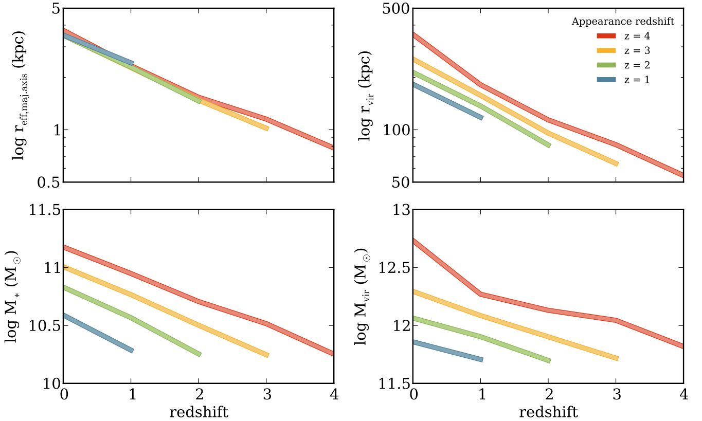
Figure 6. Growth in median size, virial radius, stellar mass, and virial mass for starforming galaxies, measured by tracing the descendants of 10^{10} M_\odot galaxies down to low redshift. Each color corresponds to galaxies which crossed the 10^{10} M_\odot mass threshold at different redshifts. For clarity, galaxies which quench before z=0 are not shown. Galaxy sizes evolve at almost the same rate as the virial radii of their parent halos: r_{\text{eff}} \propto (1+z)^{-1.2} , and r_{\text{vir}} \propto (1+z)^{-1.3} . Stellar masses increase slightly faster than virial masses: M_* \propto (1+z)^{-1.7} , and M_{\text{vir}} \propto (1+z)^{-1.2} .
