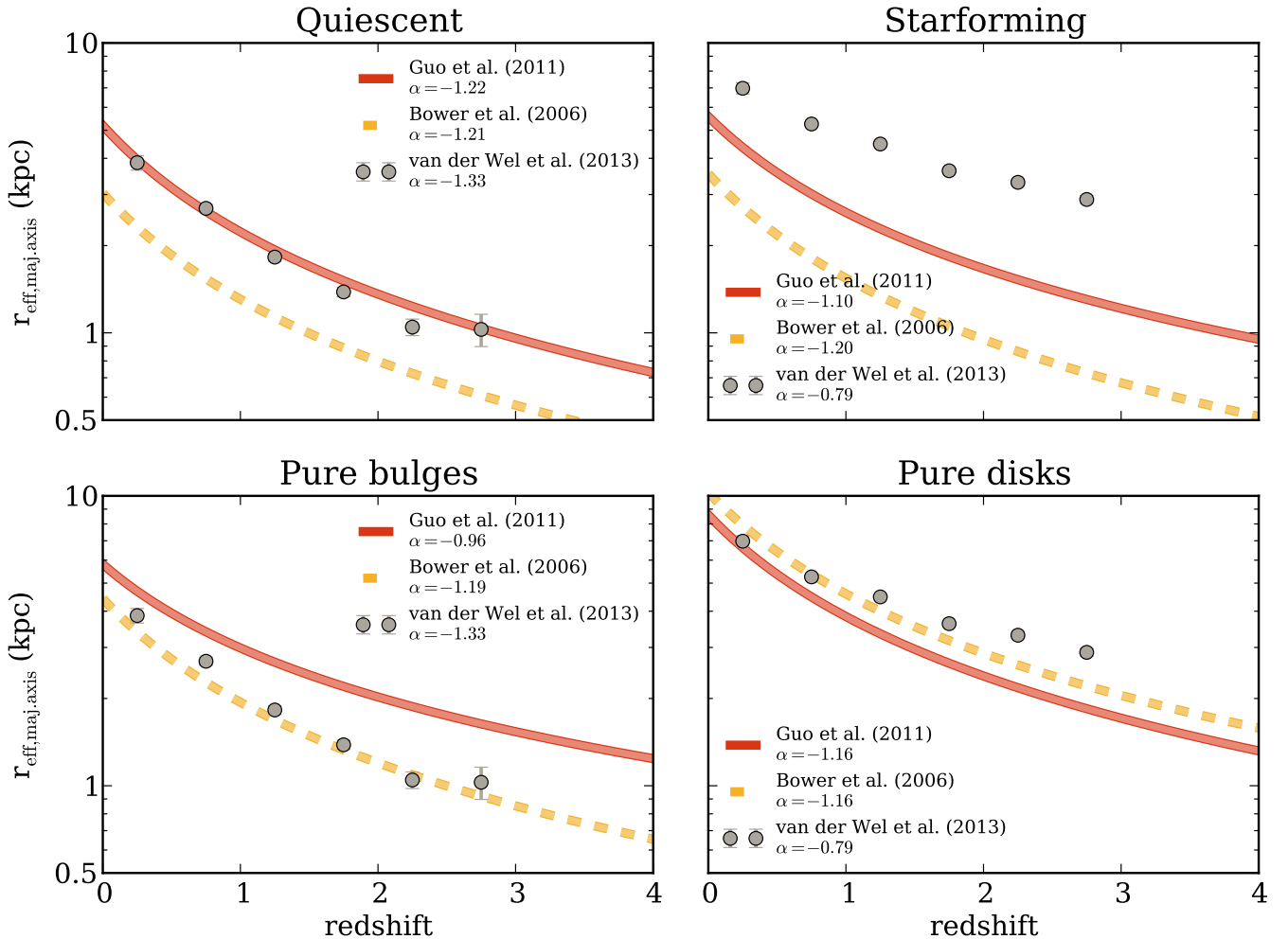
Figure 4. Top panels: median size evolution of quiescent and starforming galaxies with stellar masses 10^{10.5} < M_*/M_\odot < 10^{11} . Red (solid) and yellow (dashed) lines indicate predictions from the Guo et al. (2011) and Bower et al. (2006) models, and observed values from van der Wel et al. 2013 are indicated by the grey data points. Error bars indicate the errors on the median values. Best-fit \alpha parameters from (1+z)^\alpha power law fits are shown. The models robustly predict \alpha \approx -1.2 for quiescent galaxies, which is in good agreement with observations. The growth of starforming galaxies is somewhat overestimated in the models, and the sizes of starforming galaxies are on average a factor \sim 2-4 too small. Bottom panels: median size evolution of pure bulge and pure disk galaxies in the same mass range. In the Guo et al. (2011) model bulges grow more slowly than quiescent galaxies. In the Bower et al. (2006) model there is very little difference, possibly due to the more rapid action of disk instabilities in this SAM. Pure disk galaxies grow at a rate that is very close to that of starforming galaxies.
