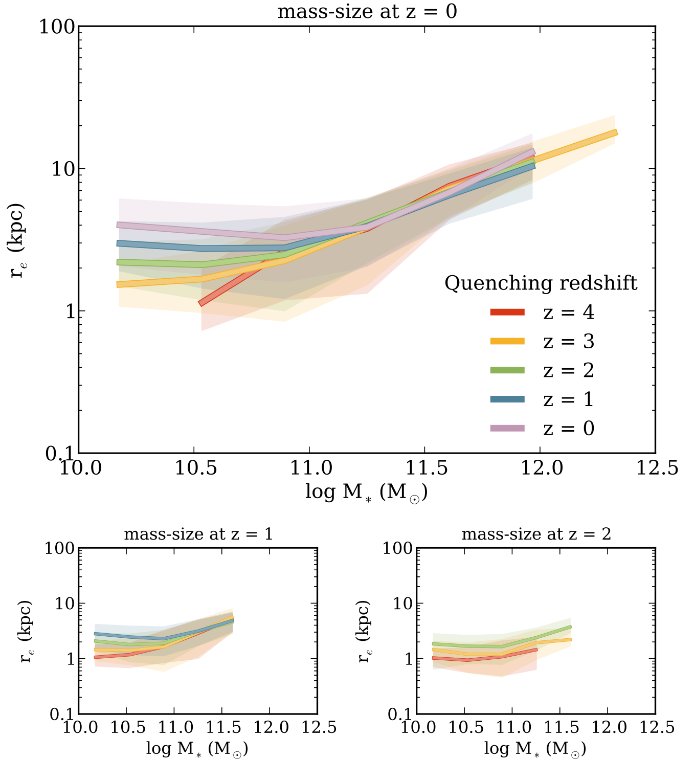
Figure 8. Running median of size as a function of stellar mass at z = 0 (top panel) and higher redshifts (lower panels) for galaxies quenched at different redshifts. At high masses ( M_* > 10^{11} M_\odot ) galaxies from different epochs lie on a tight mass-size relation. At low masses, however, there is a correlation between quenching redshift and median galaxy size: galaxies which quench early are small compared to galaxies which have quenched late.
