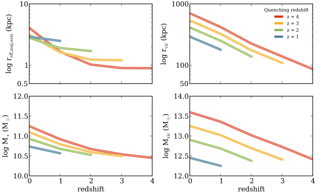
Figure 7. Growth in median size, virial radius, stellar mass, and virial mass for galaxies quenched at different redshifts. Both in the Guo and Bower models galaxies grow quite strongly in stellar mass after quenching, at a rate that is mostly independent of quenching redshift. Concurrent with this mass growth, galaxies sizes increase and virial radii and masses increase. At all redshifts older galaxies tend to be more massive and are located in larger halos. This is not the case for galaxy sizes; at high redshift the oldest galaxies tend to be the smallest, while between z = 0 and z = 1 older galaxies tend to be the largest.
