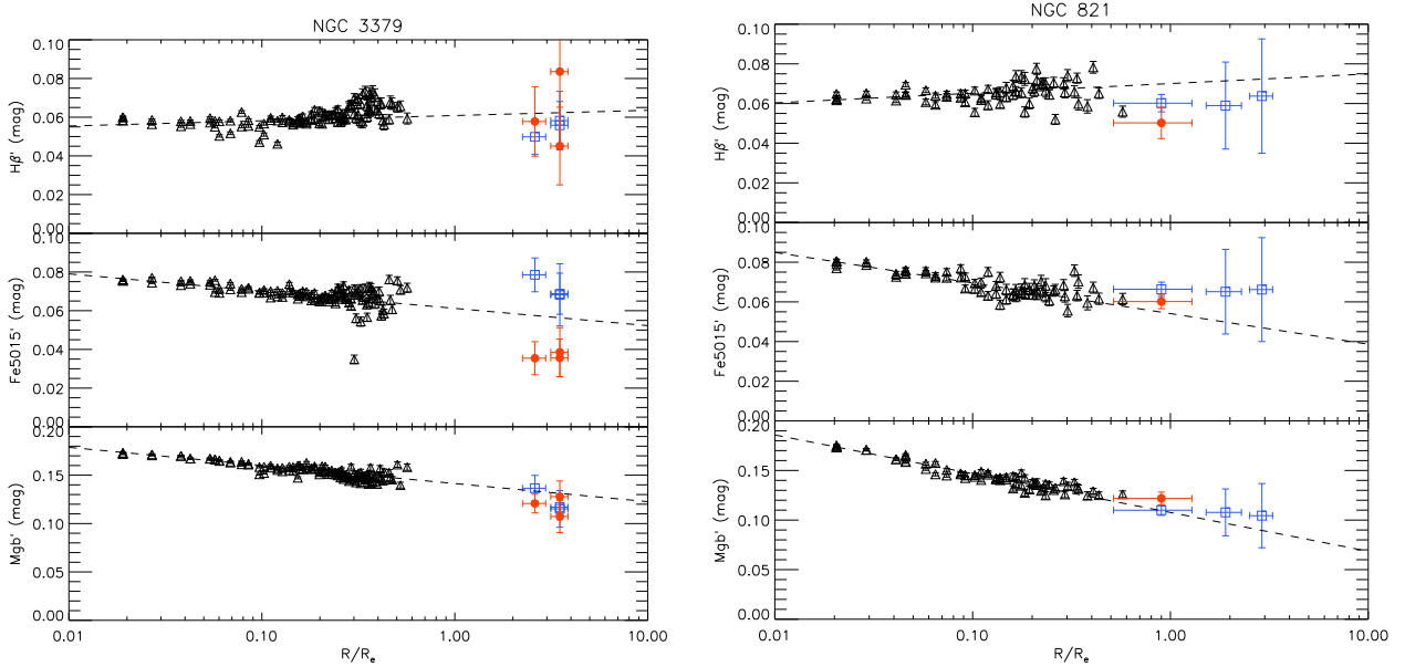
Figure 8. Line strength indices H\beta , Fe5015 and Mgb (in magnitudes) as a function of radius. Left panel: NGC 3379, right panel: NGC 821. Black triangles show indices measured on the SAURON central field, taken from a slit positioned on the major axis of the galaxy, with a width of 2 arcsec. Red filled dots show our large radii results, and the horizontal error bars denote the size of the SAURON field of view. The points at 2 and 3 R_e in NGC 821 cannot be considered reliable, probably because of continuum shape problems, and therefore are not shown here. The blue open squares denote our measurements directly from templates of single stellar population models, see text for details. Overplotted is the best fitting linear relation between index and \log(\text{radius}) , determined within R_e/4 .
