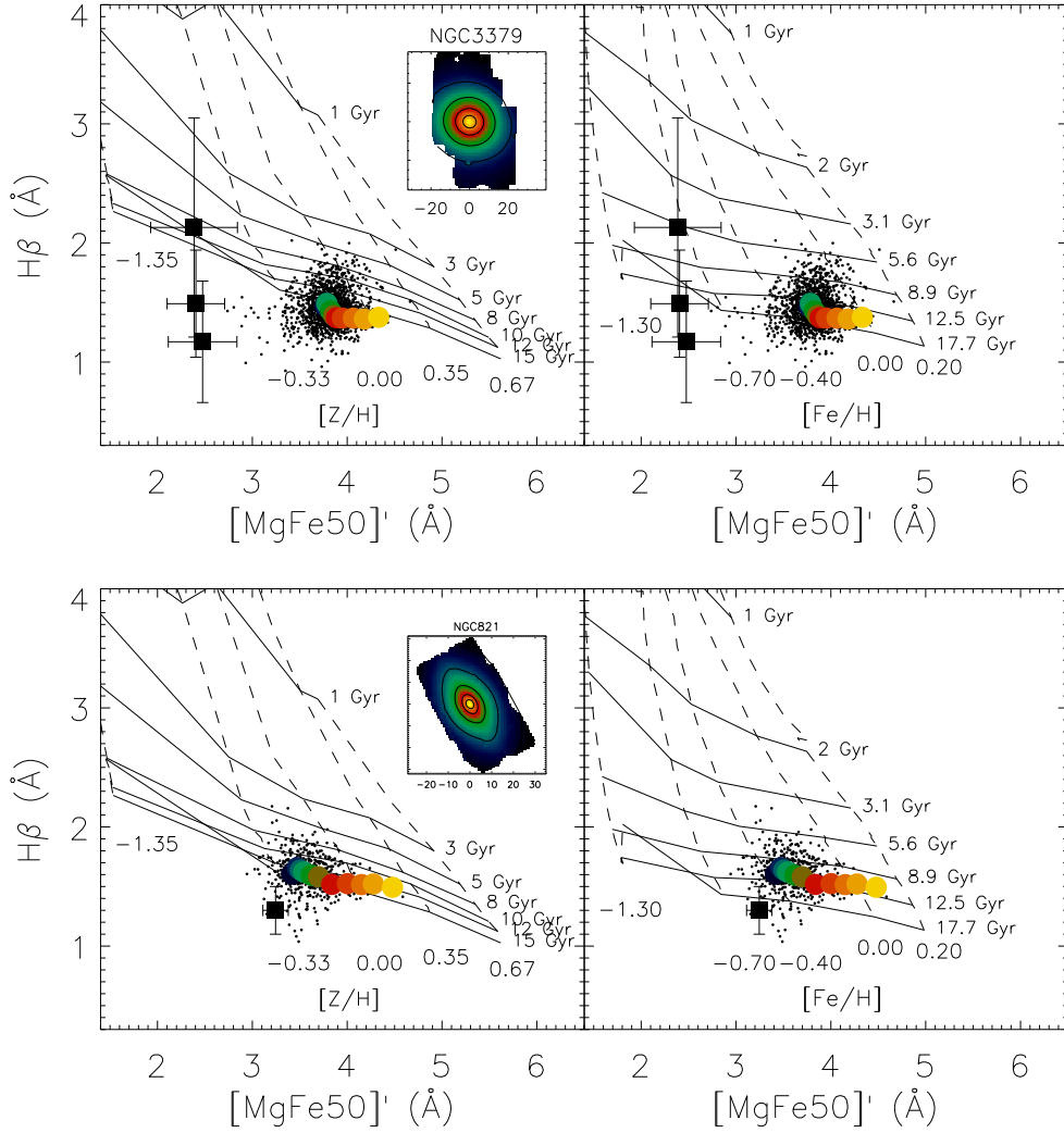
Figure 9. H\beta index against [MgFe50]' (both in \text{\AA} ) in NGC 3379 (top) and NGC 821 (bottom). Left panels show the Thomas et al. (2003) stellar population models (solid and dashed lines) and right panels the Schiavon (2007) models. Black dots indicate measurements from the SAURON central field, while the coloured dots are averaged along isophotes (see inset for colour coding). The black filled squares show the data at large radii, revealing an old (12 Gyr) and metal-poor (below 20 per cent solar metallicity) population for both models, though the uncertainties in these values are large.
