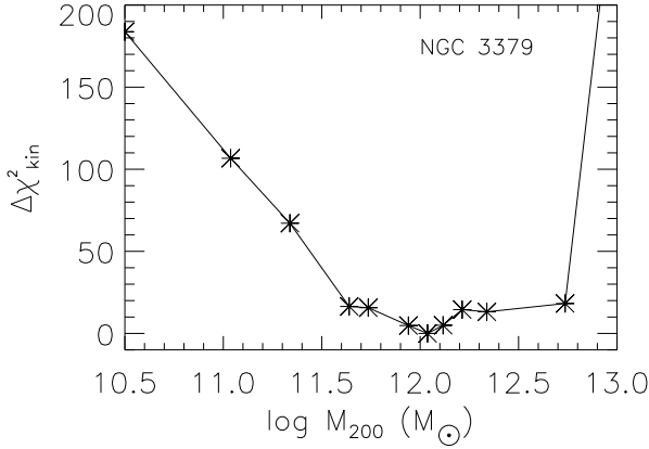
Figure 11. \Delta\chi^2 levels for the Schwarzschild models we ran for NGC 3379. The only free parameter in these models was M_{200} (total halo mass). The model without dark halo is relocated at 3 \times 10^{10} M_{\odot} , to place it within the plot.
