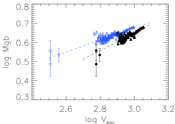
Figure 16. Mgb (in \text{\AA} ) versus local escape velocity V_{\text{esc}} (km/s) in NGC 3379. Black filled triangles denote points from the central SAURON data, while the black filled dots are our large radii data. Overplotted is the gradient fitted to the central dataset. With open symbols (in blue) we show the Mgb - V_{\text{esc}} relation calculated from our model without a halo. This relation is offset from our best-fit model and also has a different slope, illustrating the influence of the dark matter.
